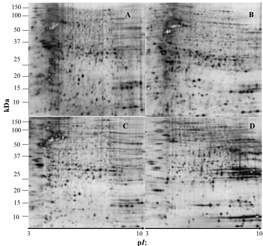
Figure 1: Two-dimensional gel electrophoresis images of MCF-7 cell and mouse liver tissue proteomes isolated by different protein isolation methodologies. Aqueous phase proteins isolated by using chloroform-assisted protein isolation (ChIAPI) method from MCF-7 cells (A) and mouse liver tissue (D). MCF-7 cell total soluble proteome isolated by detergent lysis followed by sonication (B), and by French Pressure Cell Press(C).
